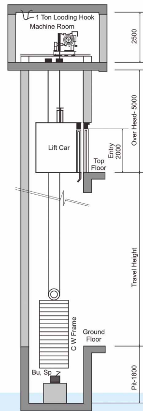
HOISTWAY ELEVATION DRAWING
